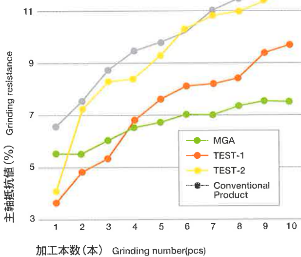
抵抗値比較 Comparison of resistance value
